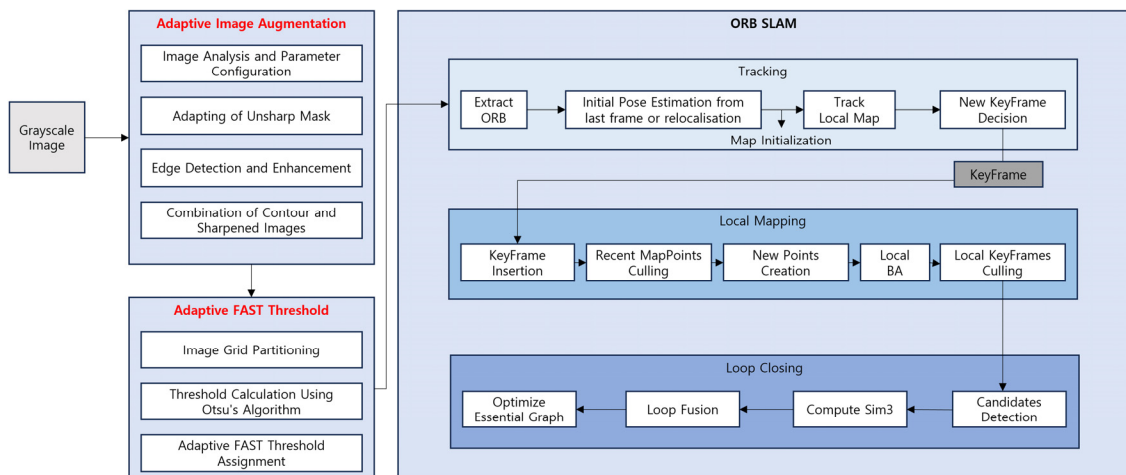
[Fig. 2] Proposed method pipeline
